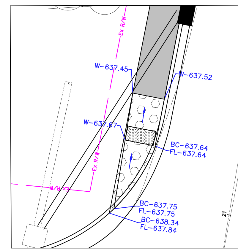
CURB RAMP DETAIL F ODOT TYPE B3 RAMP NOT TO SCALE
