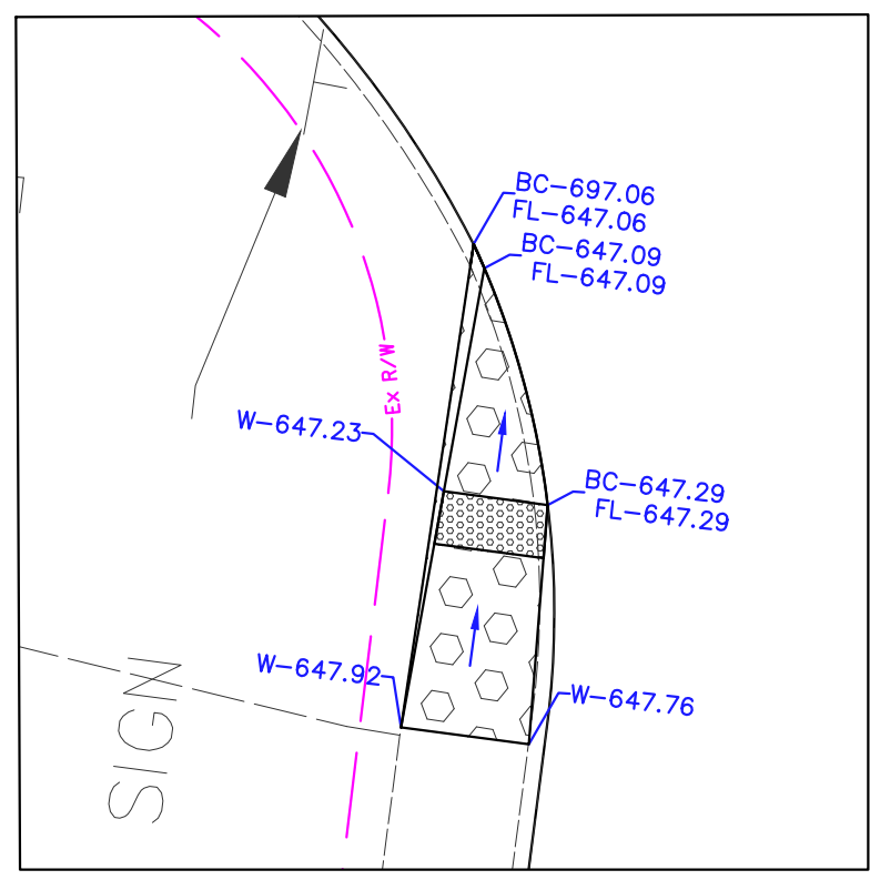
CURB RAMP DETAIL C ODOT TYPE B3 RAMP NOT TO SCALE
