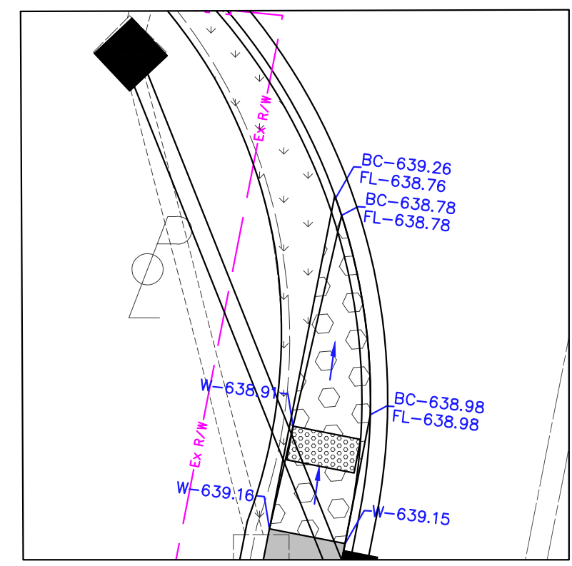
CURB RAMP DETAIL E ODOT TYPE B3 RAMP NOT TO SCALE
