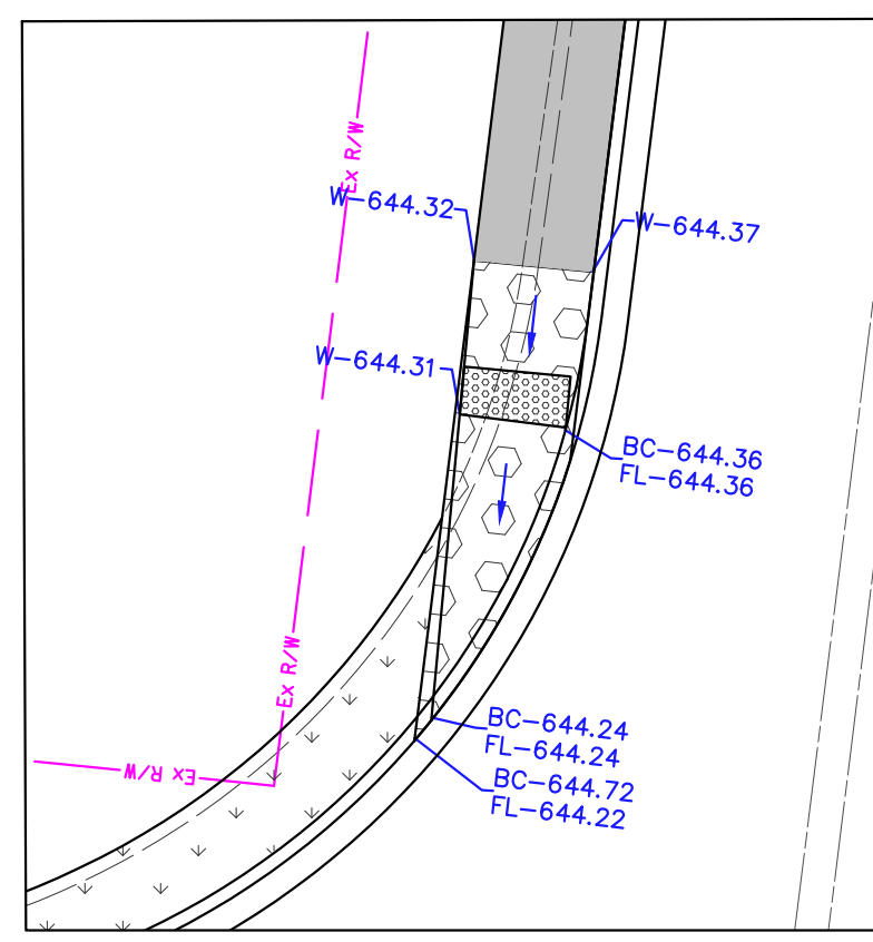
CURB RAMP DETAIL D ODOT TYPE B3 RAMP NOT TO SCALE
