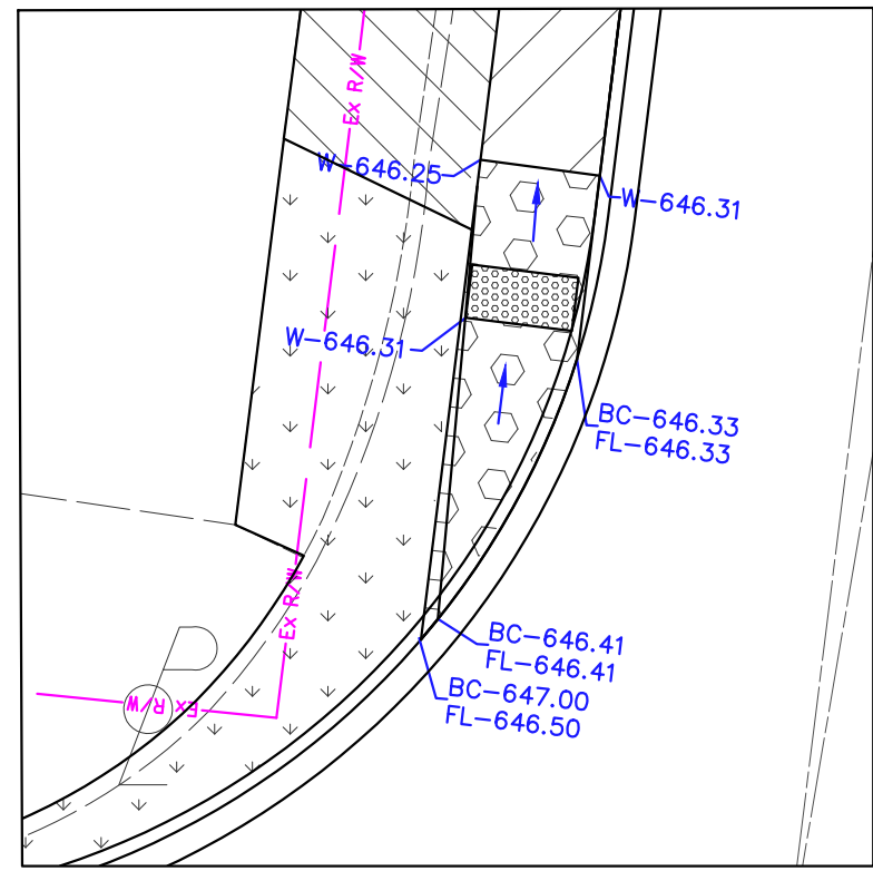
CURB RAMP DETAIL B ODOT TYPE B3 RAMP NOT TO SCALE
