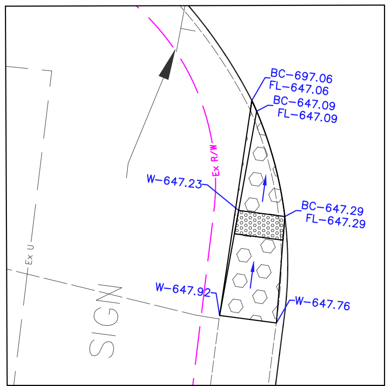
CURB RAMP DETAIL A ODOT TYPE B3 RAMP NOT TO SCALE
